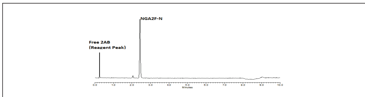
Figure 1 - UHPLC Results: 3 - 6 pmol (1 \mu l, aqueous) of the 2-AB-labeled 4 glycan was injected on a UHPLC System (Waters ACQUITY H Class) utilizing a 10-minute method under the conditions below:
