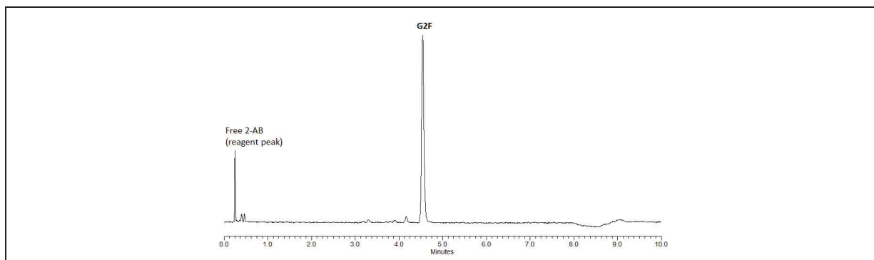
Figure 1 - UHPLC Results: 3–6 pmol (1 \mu L, aqueous) of the 2-AB-labeled 4 glycan was injected on a UHPLC System (Waters ACQUITY H Class) utilizing a 10-minute method under the conditions below:
