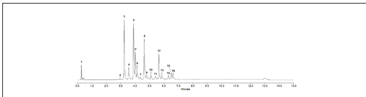
Figure 1 - UPLC Results: 1 \mu L, aqueous of the InstantPC-labeled glycan was injected on a Waters ACQUITY UPLC H Class System utilizing a 15-minute method under the conditions below (see Table 1 for peak ID; the number of peaks observed depends on the running conditions employed):
